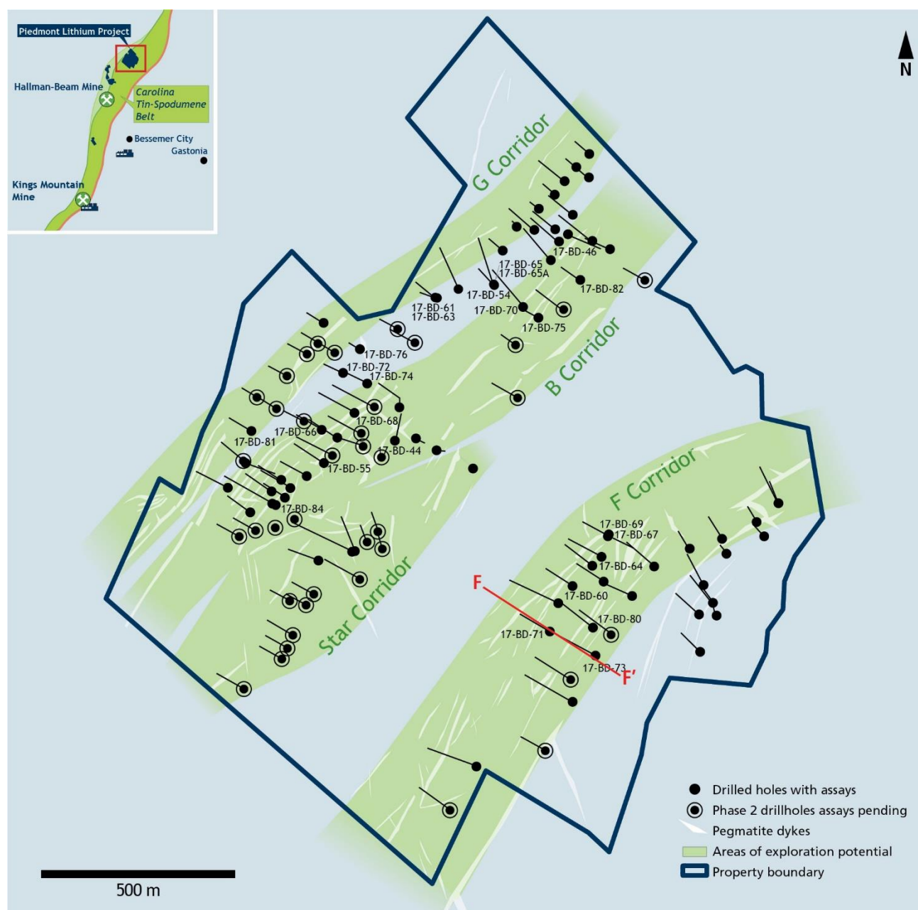
Figure 2: Piedmont Lithium Phase 2 Drillhole Location Map with Corridors
