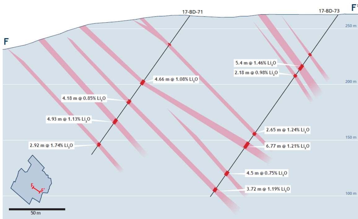
Figure 3: Piedmont Lithium F Corridor Cross Section
